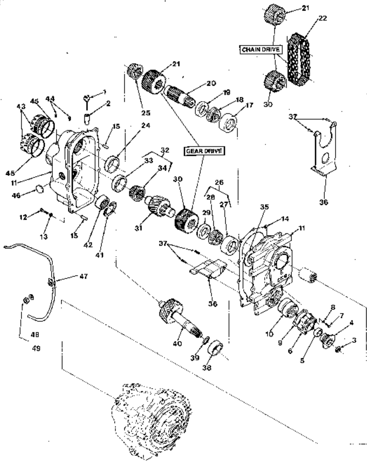
Figure 12. V-Drive Assembly
