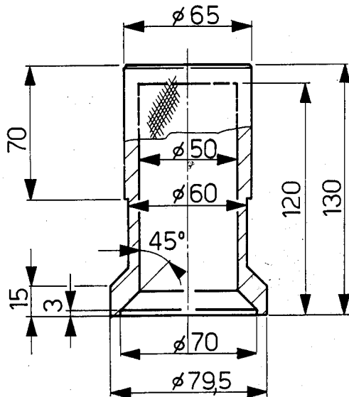
Attrezzo / Tool: 15751990117 (cuscinetto / bearing 50 - 63 - 66 - 79)
