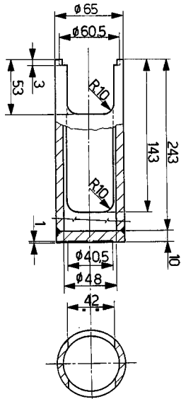
Attrezzo / Tool: 15751990117 (cuscinetto / bearing 50 - 63 - 66 - 79)
