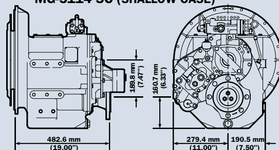
MG-5114 SC (SHALLOW CASE)
